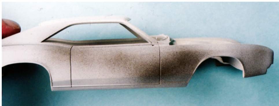
Figure 11.1: Once your basic bodywork is finished and primed, apply a light coat of very dark lacquer (preferably black) over the primed areas that cover your bodywork. The purpose of applying a guide coat is to detect high and low spots in your bodywork when the guide coat is sanded.
