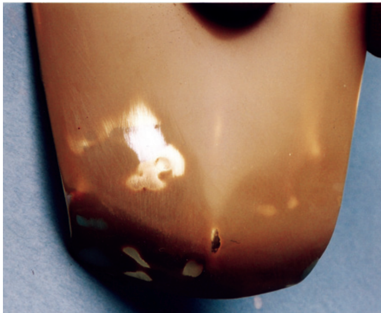
Figure 10.59: Apply more Variprime, let it cure, and then use a coarse sanding stick to sand the surface again. In this view, there is an obvious high spot that remains following the steps in Figure 10.58. Again, lightly tap around this high spot, but be careful not to work the spot too much or you’ll have a low spot!
