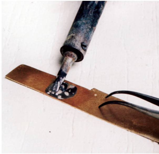
Figure 10.10: . . . in the deposition of the solder on the surface. Spread the solder around a bit, making sure that the solder flows out easily, and is shiny at the completion of this operation.
